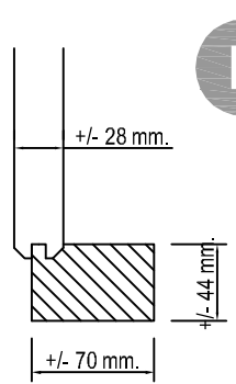
Shinglesdak Schindeldach Shingleroof
